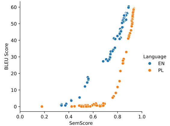
Figure 4: Distribution of BLEU and SemScore for English and Polish translations across 144 fine-tuned models.
