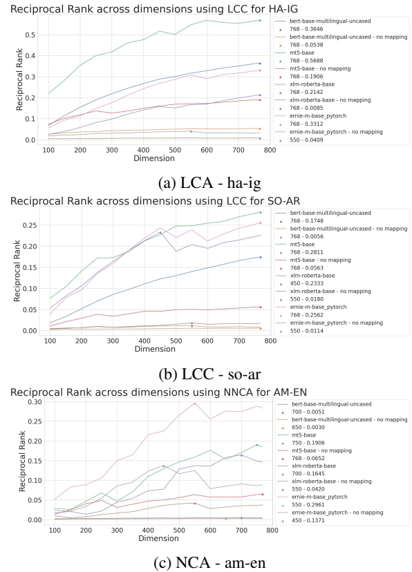
Figure 3: Reciprocal rank across dimensions using LCA, LCC and NCA for different language pairs
