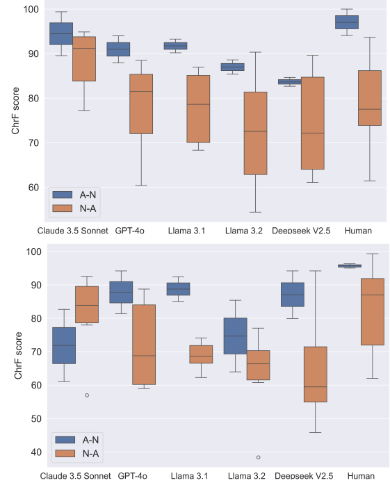
Figure 6: ChrF scores in N-A and A-N order languages. Up: to English; down: to LR languages
